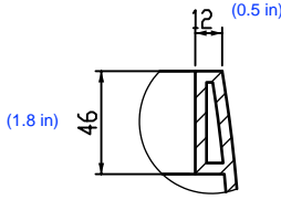
DETAIL CD
