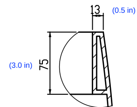
DETAIL CH
